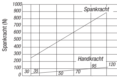
Trekspanner K0910.3240...
